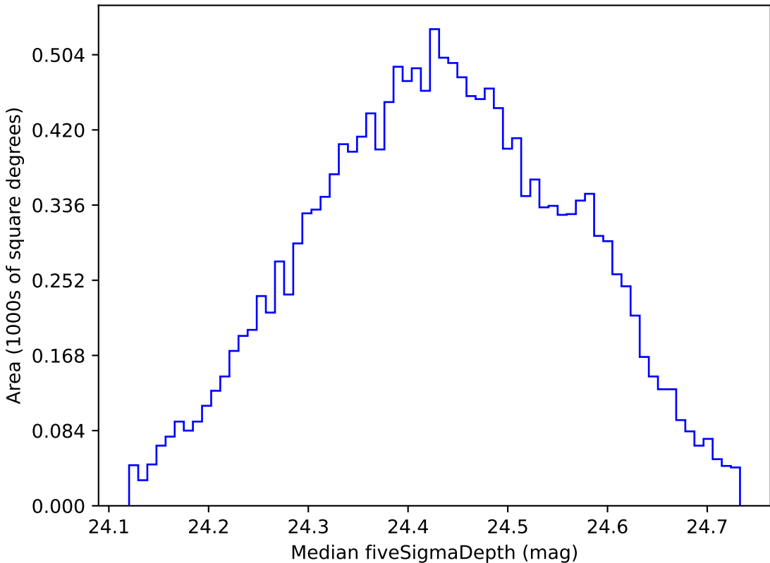
too_100_4v3.4_10yrs WFD g band: Median fiveSigmaDepth
