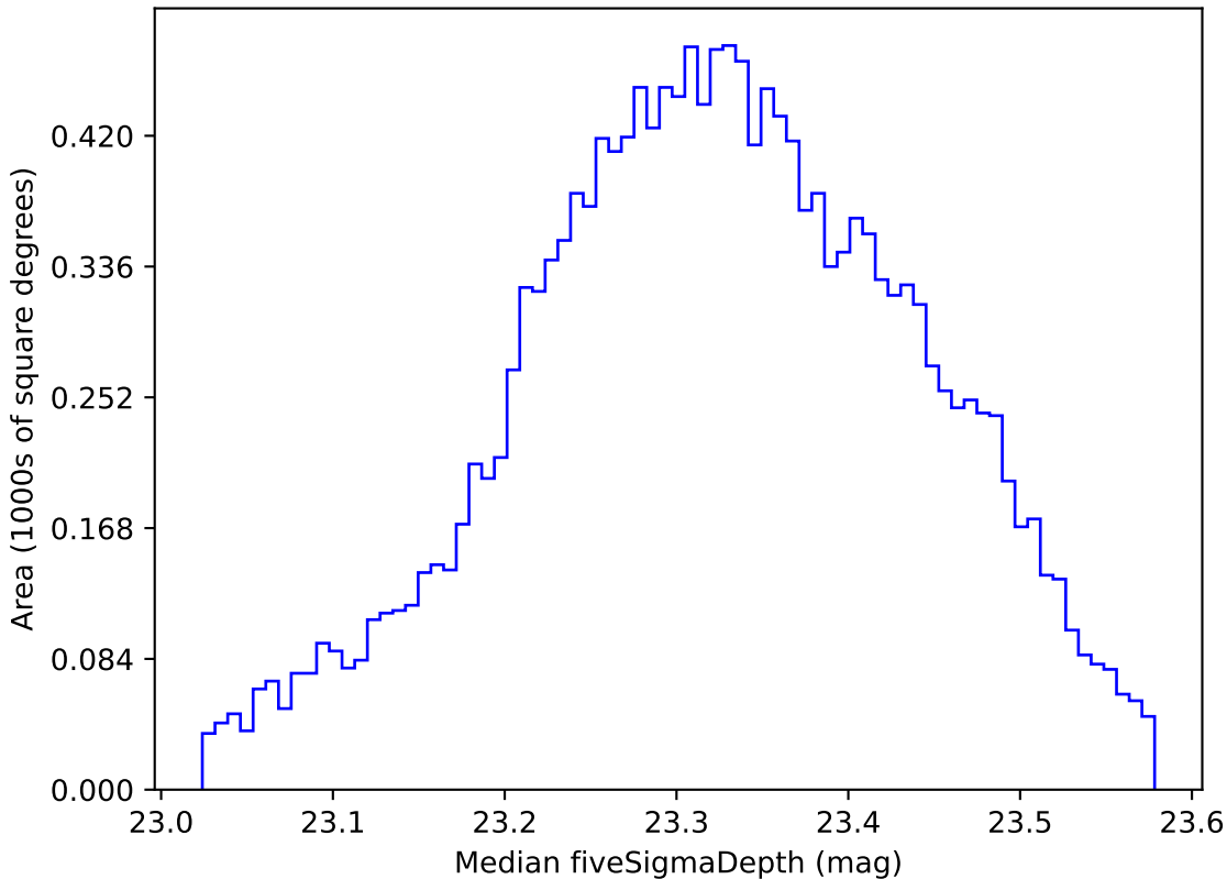
too_100_4v3.4_10yrs WFD all bands: Median fiveSigmaDepth
