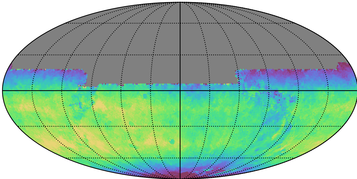
too_100_4v3.4_10yrs All sky y band: Median fiveSigmaDepth
