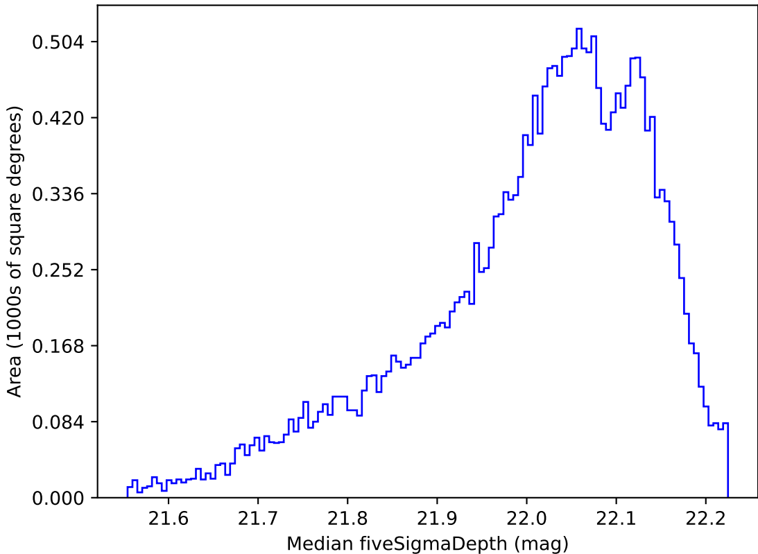
too_100_4v3.4_10yrs All sky y band: Median fiveSigmaDepth
