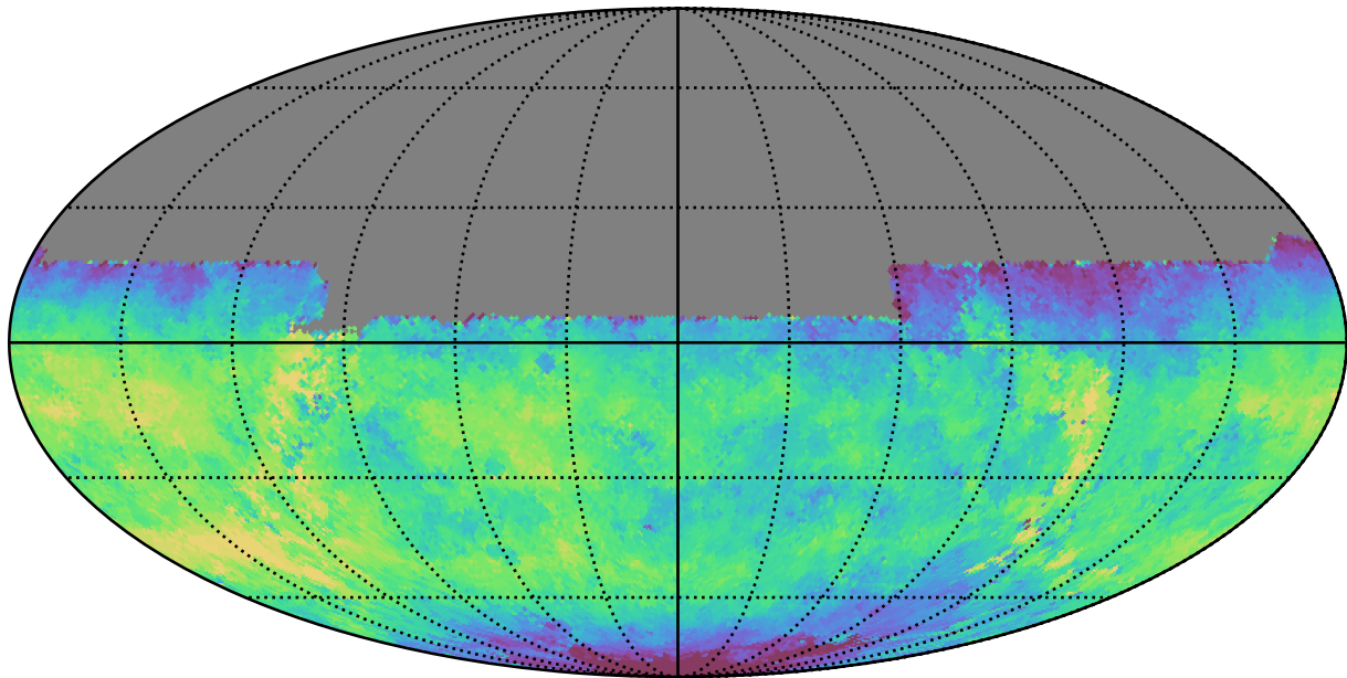
too_100_4v3.4_10yrs All sky u band: Median fiveSigmaDepth
