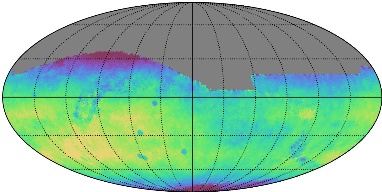
too_100_4v3.4_10yrs All sky r band: Median fiveSigmaDepth
