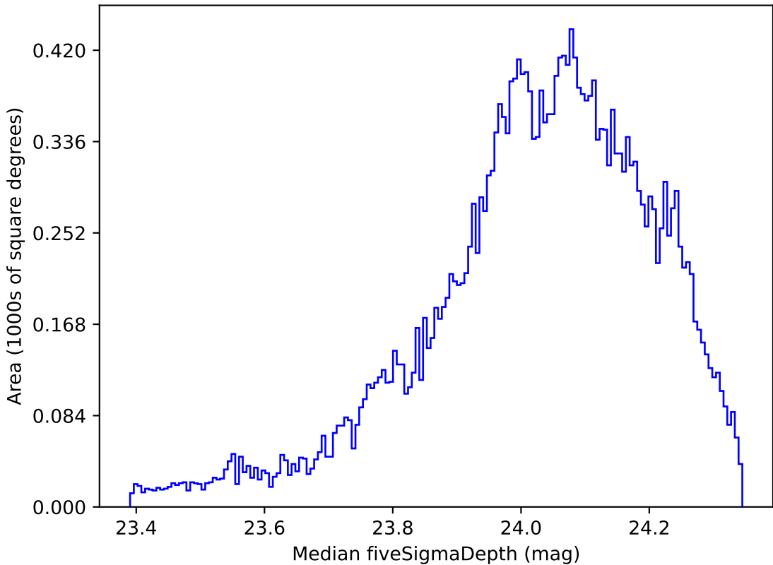
too_100_4v3.4_10yrs All sky r band: Median fiveSigmaDepth
