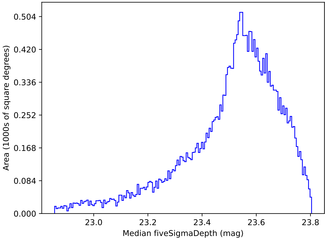
too_100_4v3.4_10yrs All sky i band: Median fiveSigmaDepth
