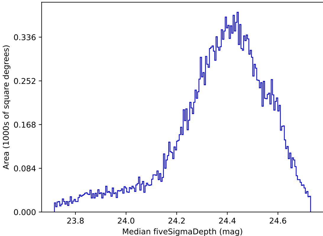
too_100_4v3.4_10yrs All sky g band: Median fiveSigmaDepth
