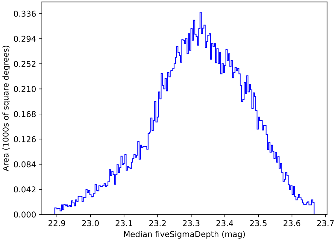
too_100_4v3.4_10yrs All sky all bands: Median fiveSigmaDepth
