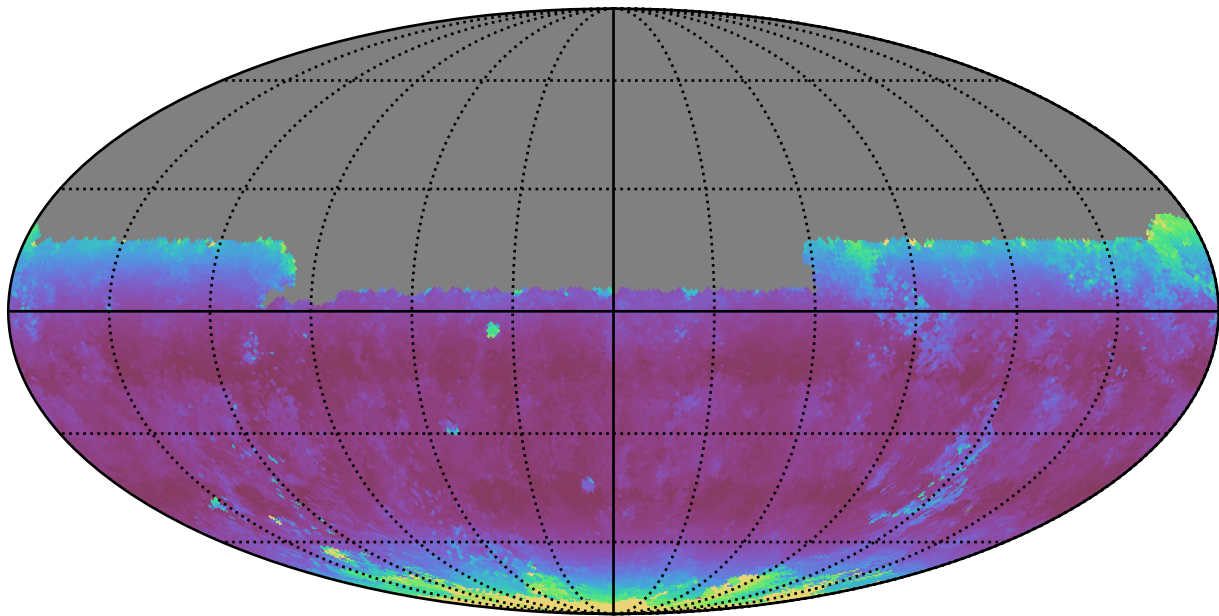
too_100_4v3.4_10yrs Yr 1 y band: Median airmass
