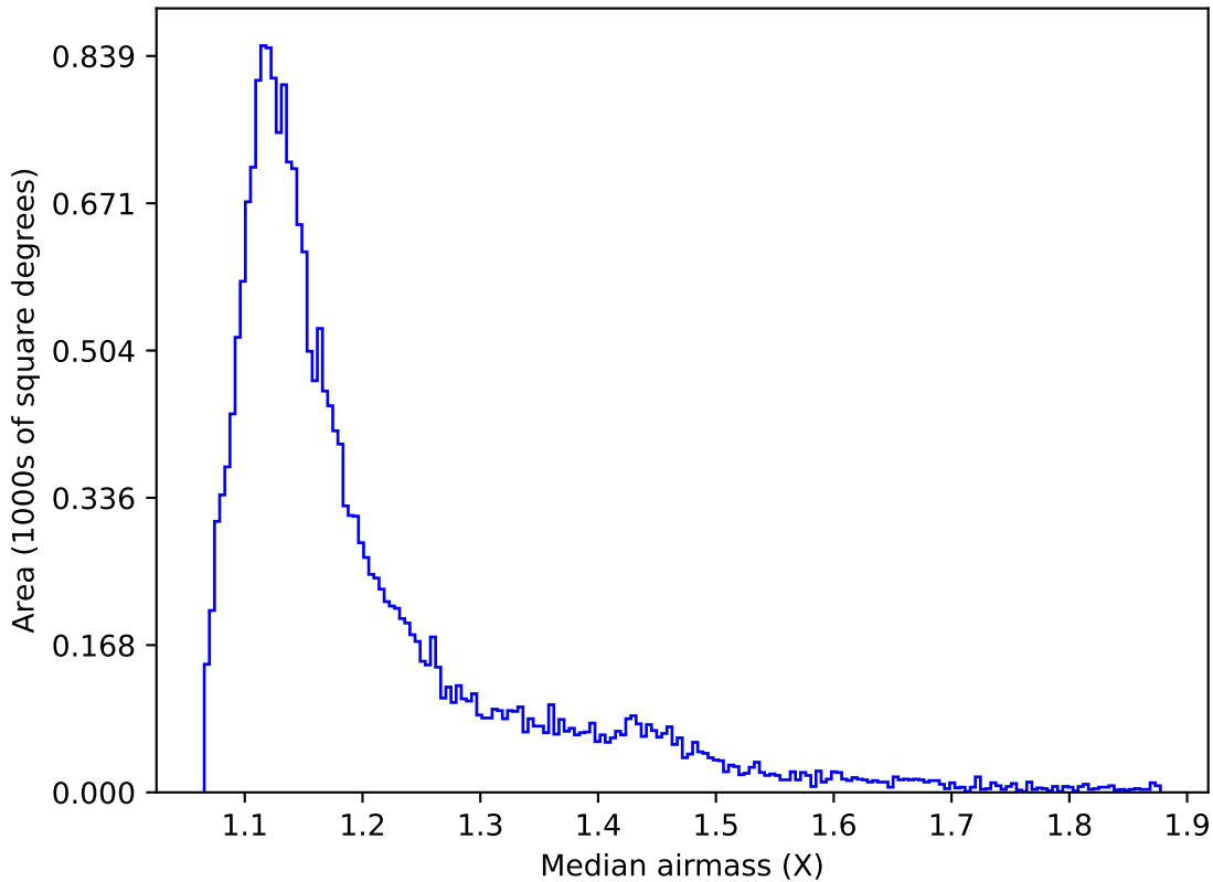
too_100_4v3.4_10yrs Yr 1 y band: Median airmass
