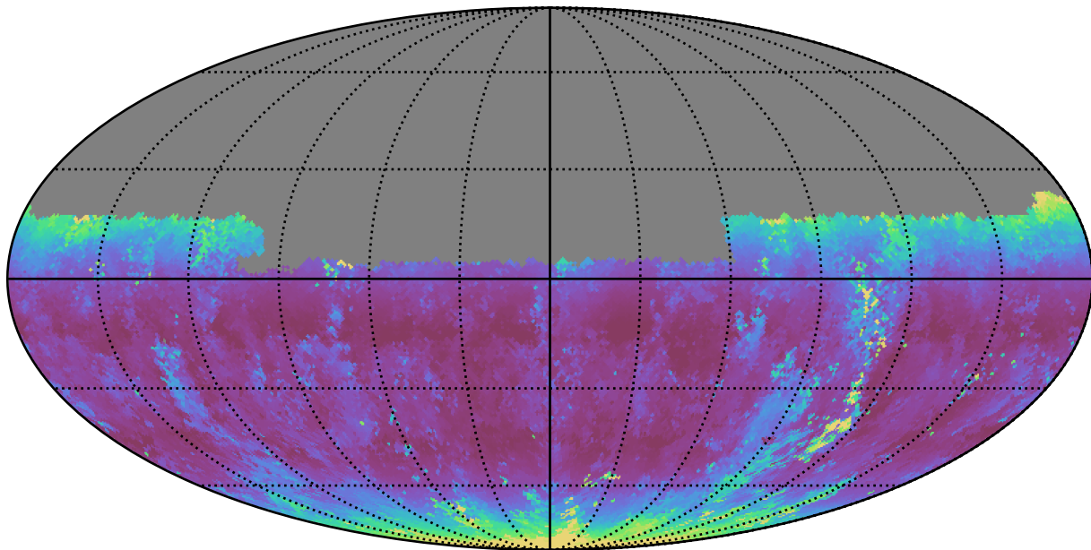
too_100_4v3.4_10yrs Yr 1 u band: Median airmass
