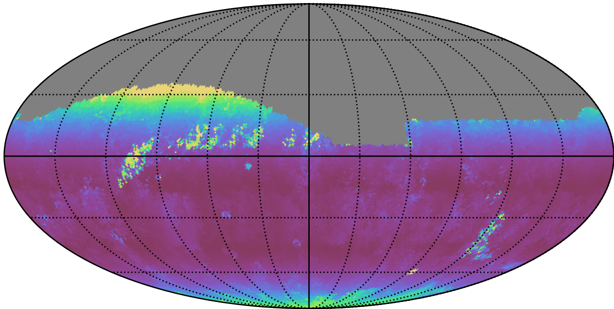
too_100_4v3.4_10yrs Yr 1 r band: Median airmass
