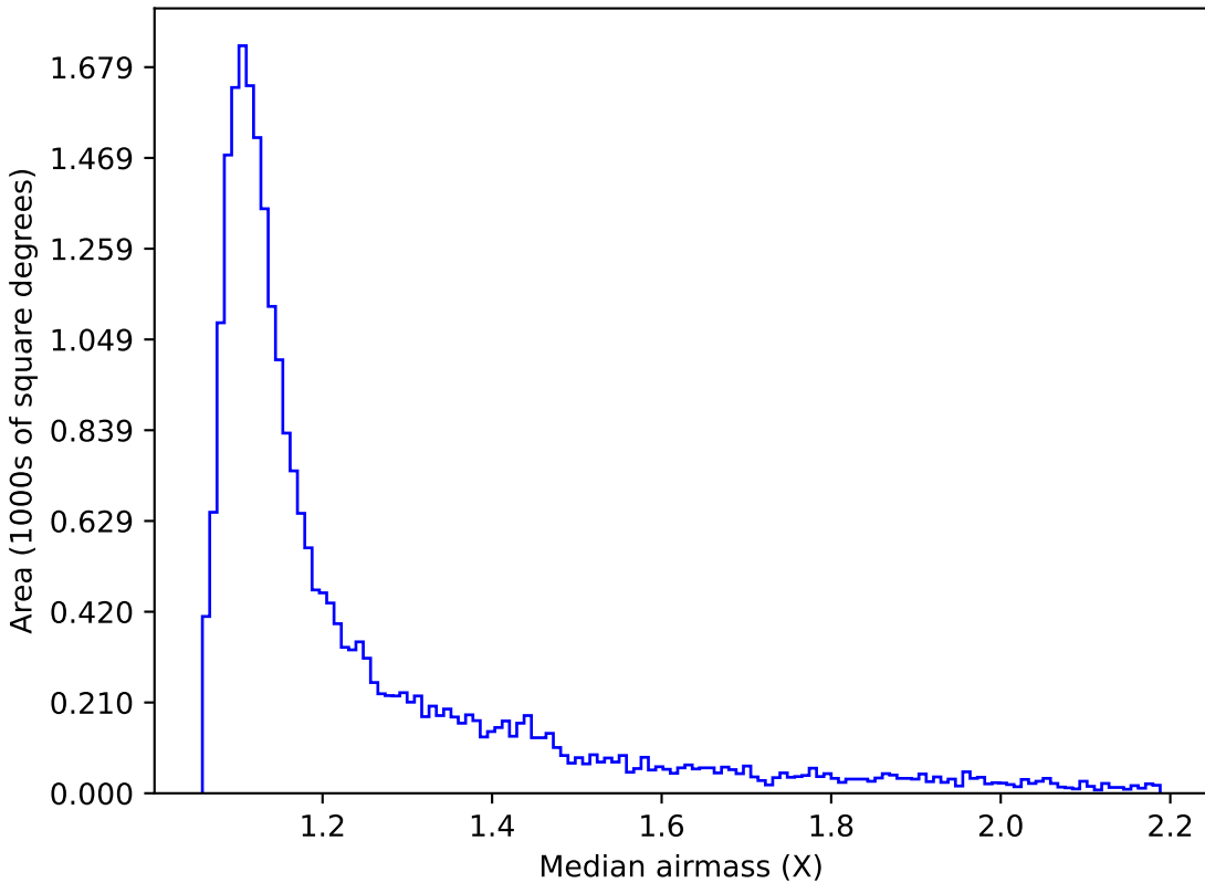
too_100_4v3.4_10yrs Yr 1 i band: Median airmass
