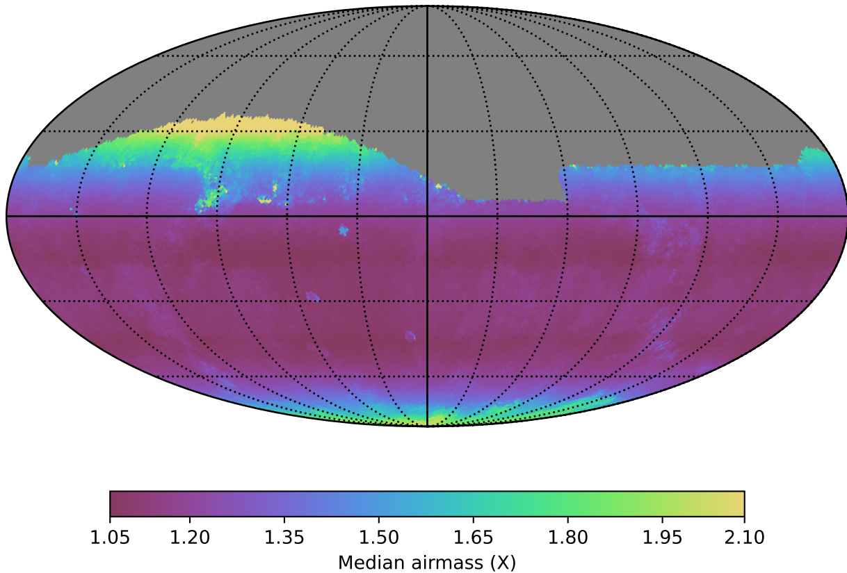
too_100_4v3.4_10yrs Yr 1 all bands: Median airmass
