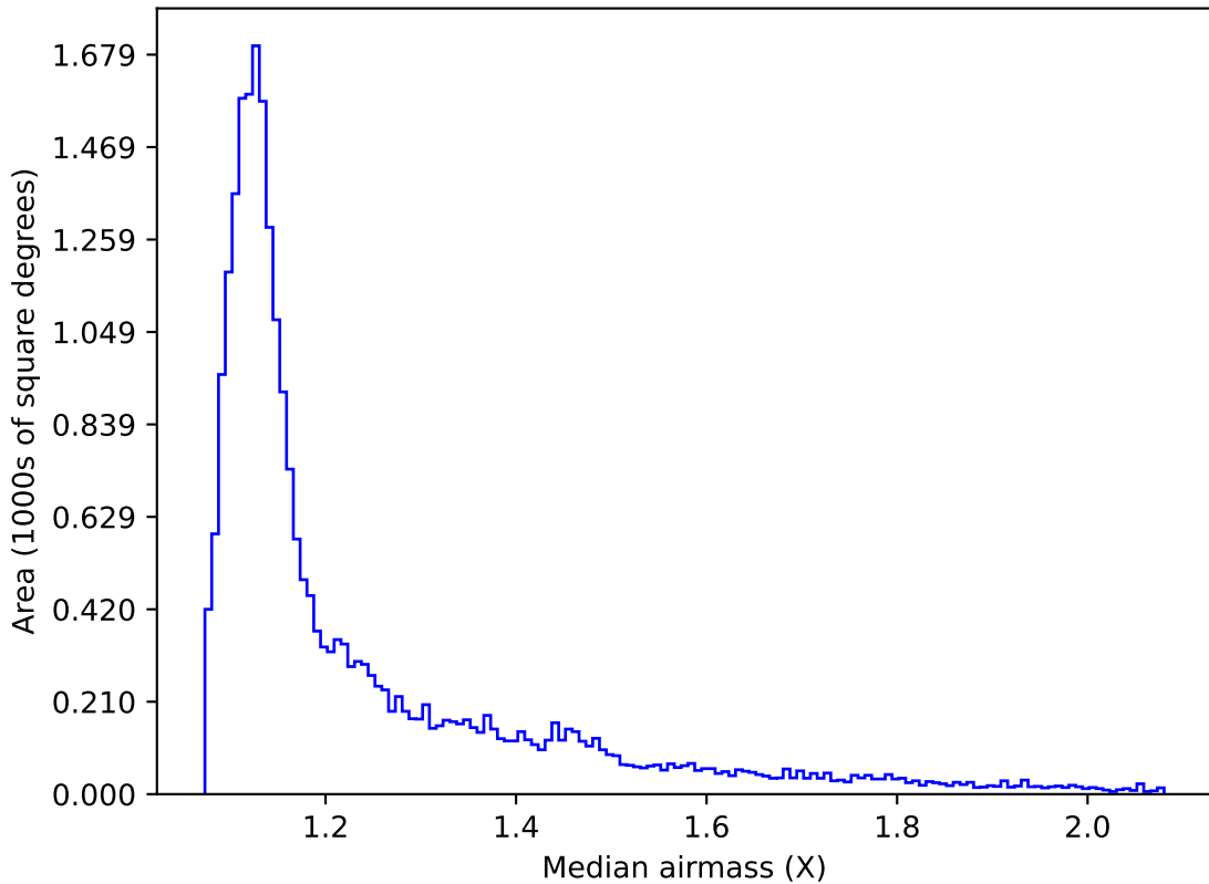
too_100_4v3.4_10yrs Yr 1 all bands: Median airmass
