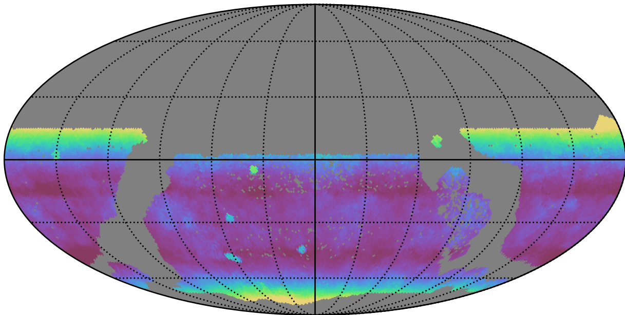
too_100_4v3.4_10yrs WFD y band: Median airmass
