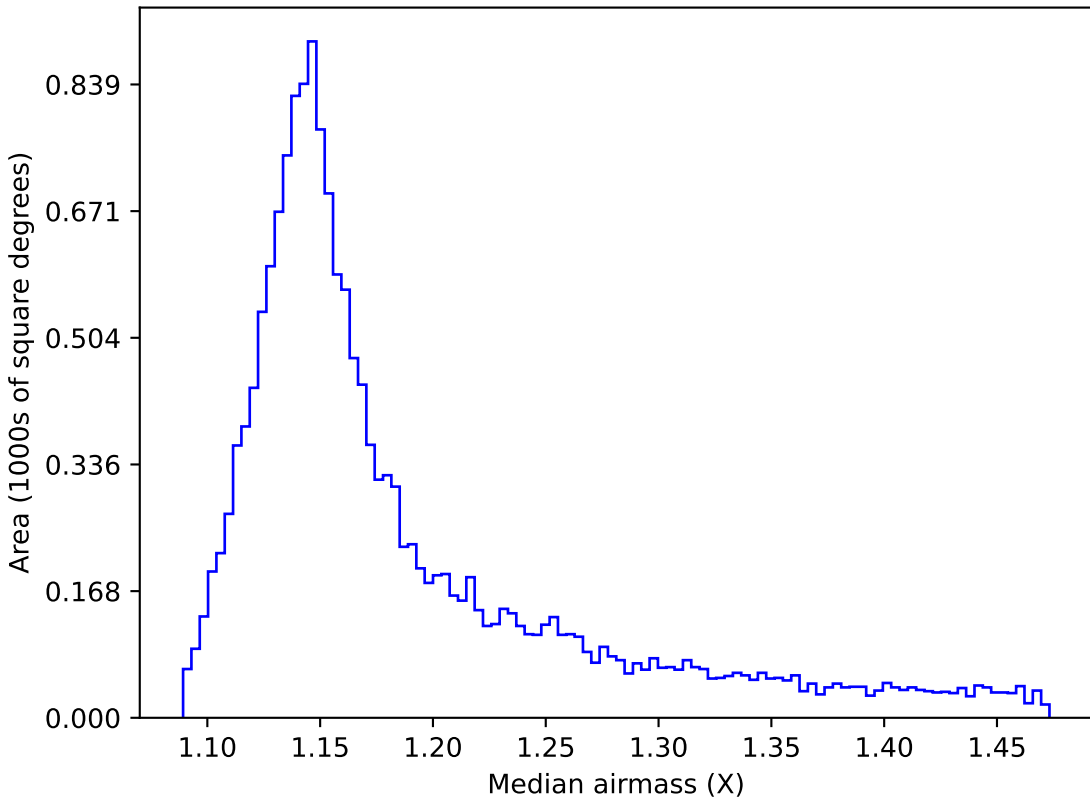
too_100_4v3.4_10yrs WFD y band: Median airmass
