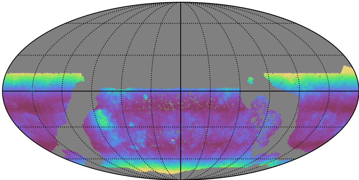
too_100_4v3.4_10yrs WFD u band: Median airmass
