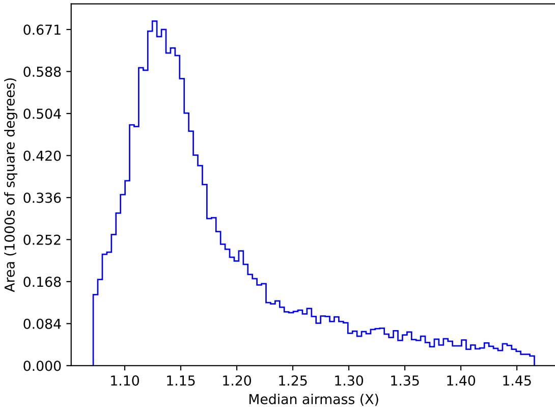
too_100_4v3.4_10yrs WFD u band: Median airmass
