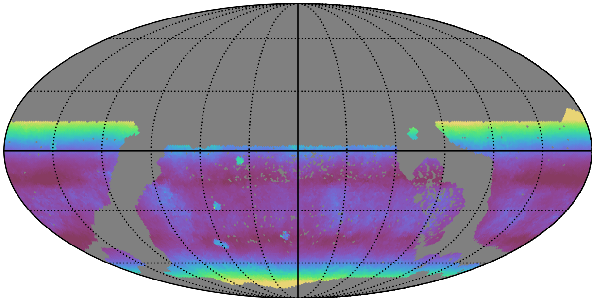
too_100_4v3.4_10yrs WFD r band: Median airmass
