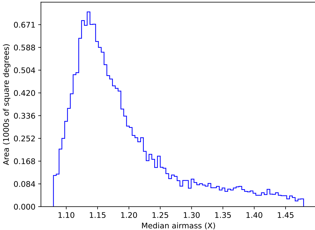
too_100_4v3.4_10yrs WFD g band: Median airmass
