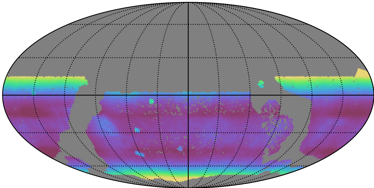
too_100_4v3.4_10yrs WFD all bands: Median airmass
