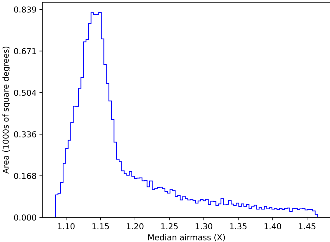
too_100_4v3.4_10yrs WFD all bands: Median airmass
