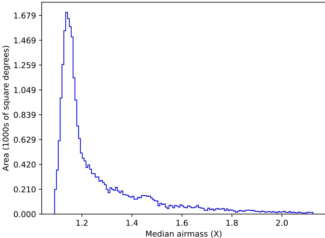
too_100_4v3.4_10yrs All sky z band: Median airmass
