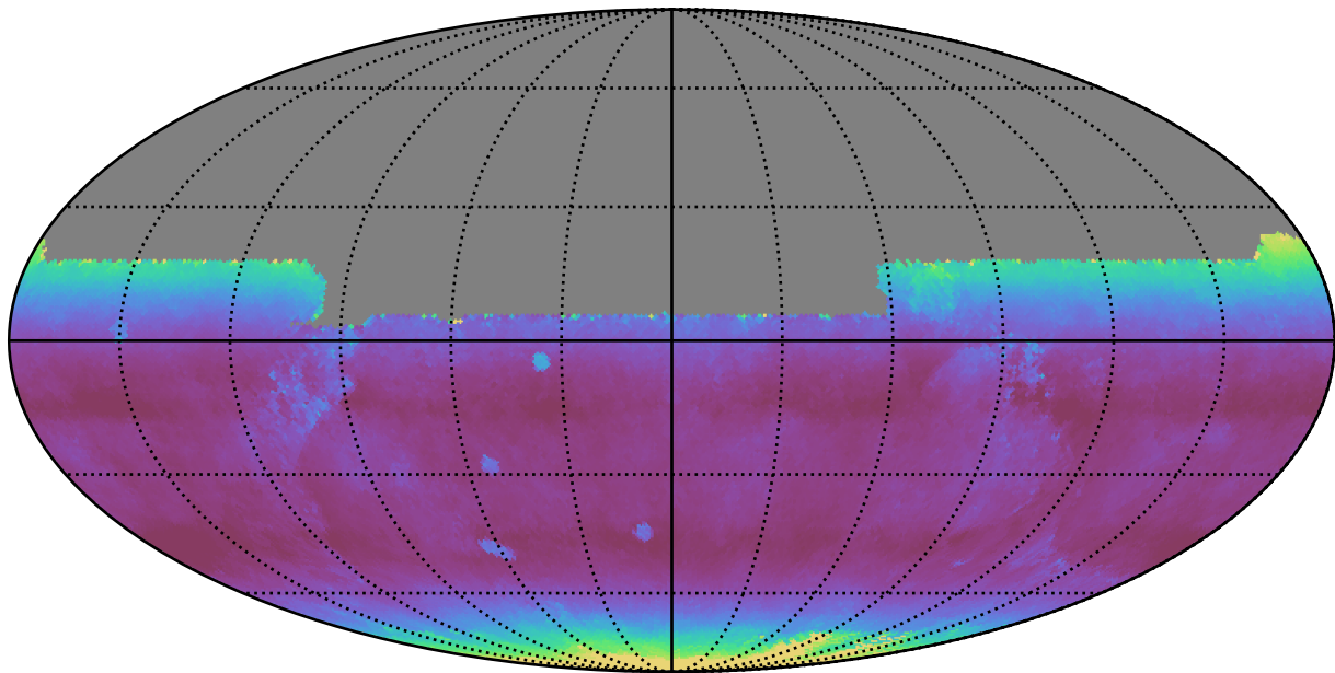
too_100_4v3.4_10yrs All sky y band: Median airmass
