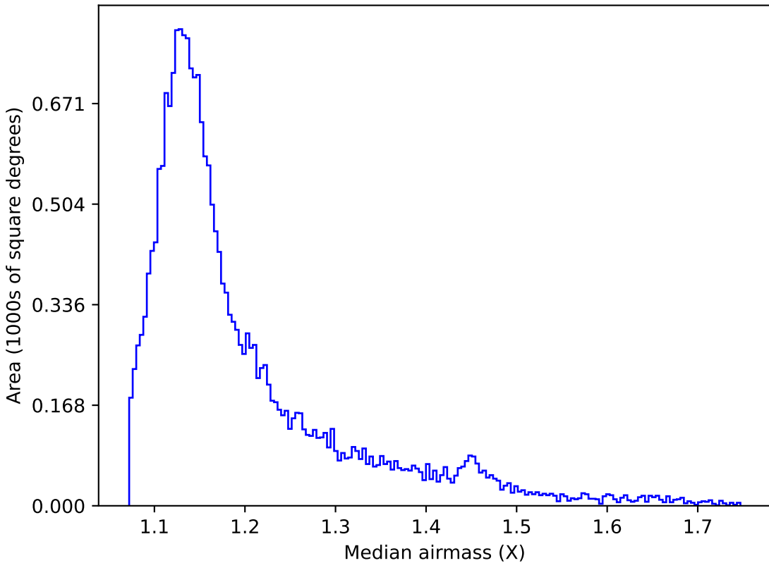
too_100_4v3.4_10yrs All sky u band: Median airmass
