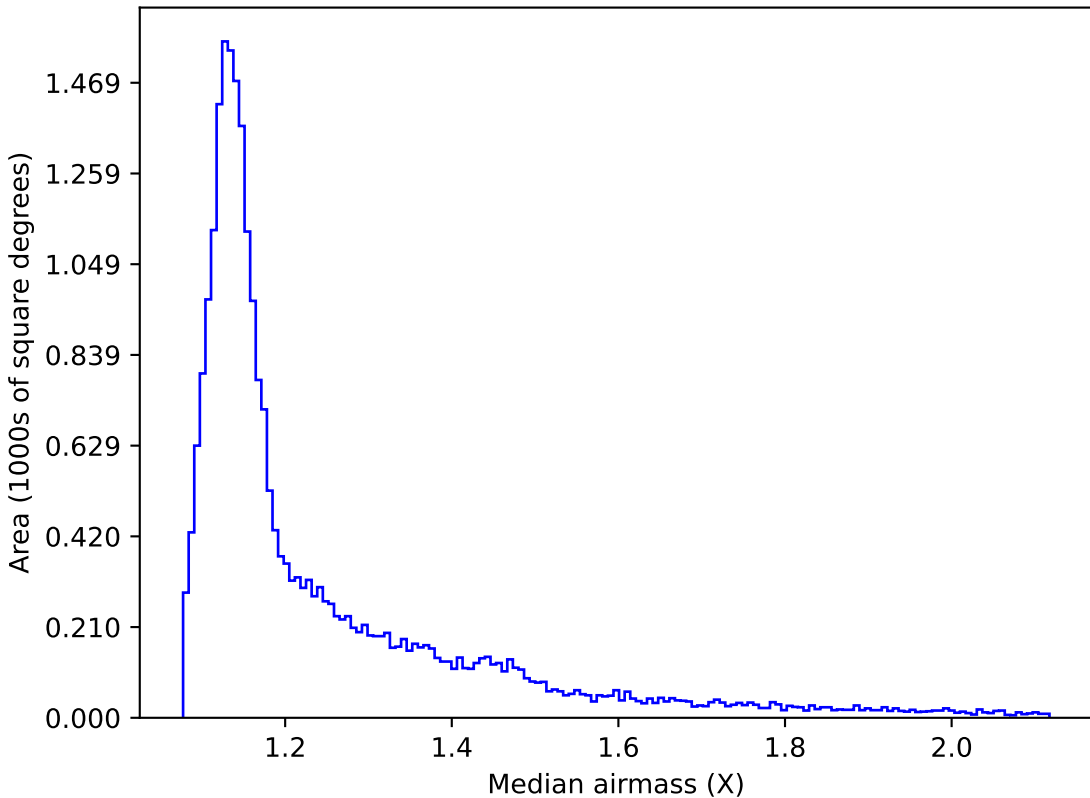
too_100_4v3.4_10yrs All sky r band: Median airmass
