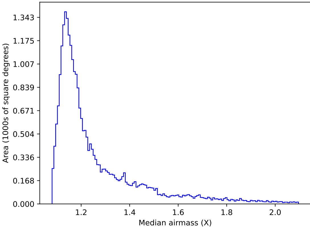
too_100_4v3.4_10yrs All sky g band: Median airmass
