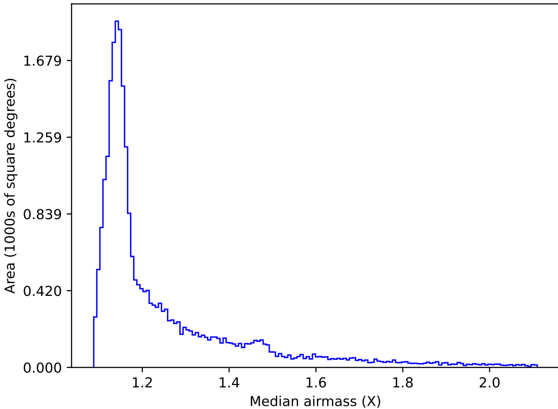
too_100_4v3.4_10yrs All sky all bands: Median airmass
