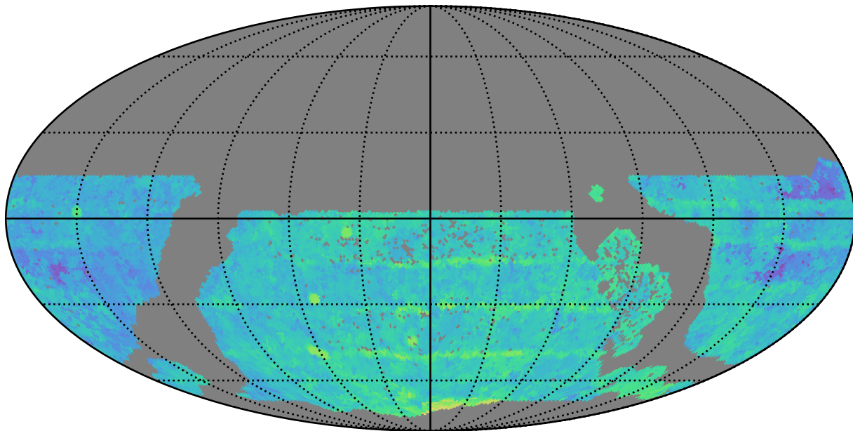
too_100_4v3.4_10yrs WFD z band: Median Season Length
