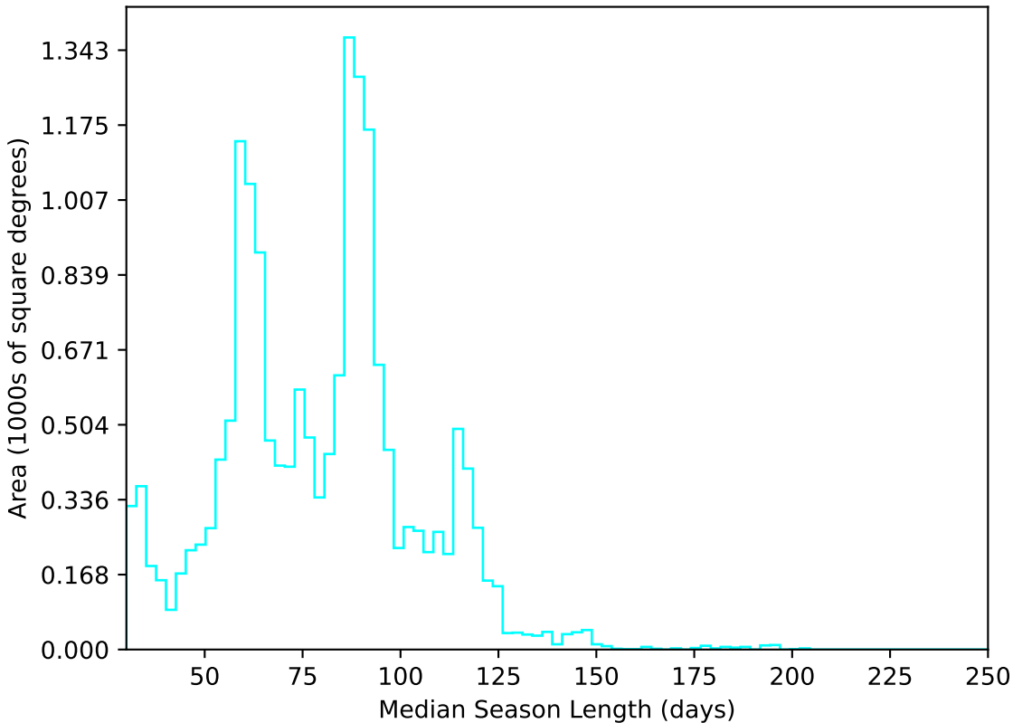
too_100_4v3.4_10yrs WFD u band: Median Season Length
