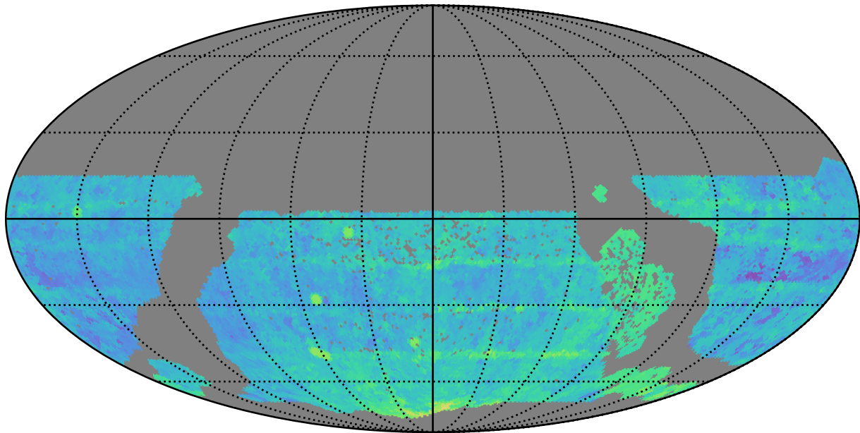
too_100_4v3.4_10yrs WFD r band: Median Season Length
