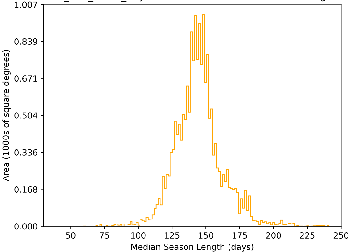
too_100_4v3.4_10yrs WFD r band: Median Season Length
