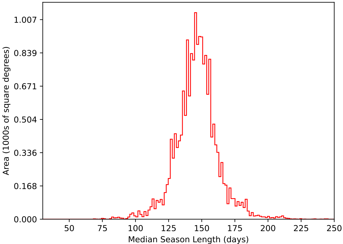
too_100_4v3.4_10yrs WFD i band: Median Season Length
