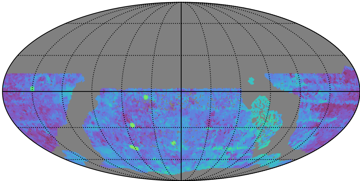
too_100_4v3.4_10yrs WFD g band: Median Season Length
