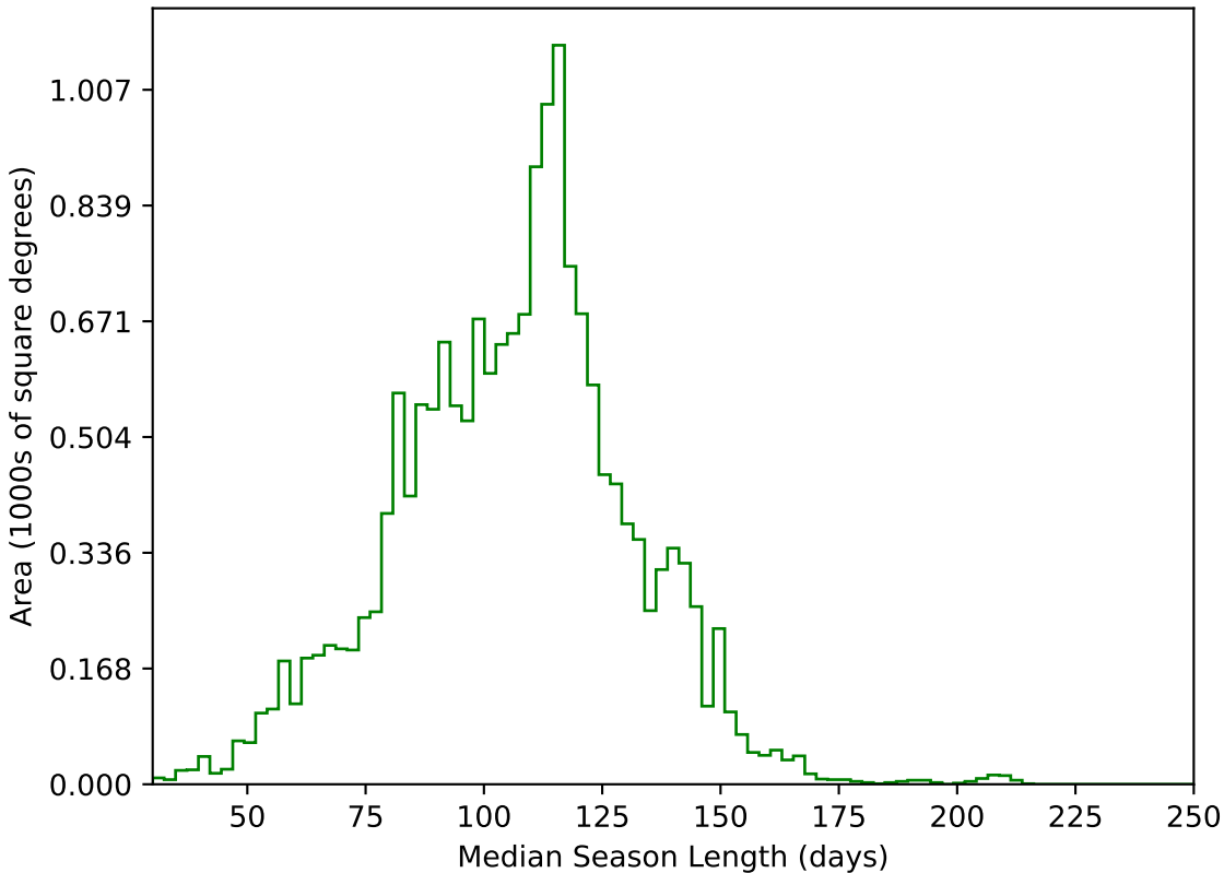
too_100_4v3.4_10yrs WFD g band: Median Season Length
