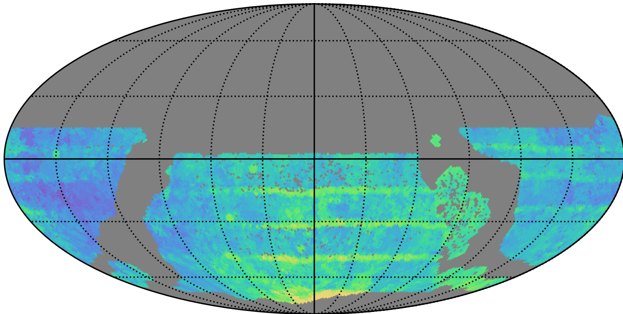
too_100_4v3.4_10yrs WFD all bands: Median Season Length
