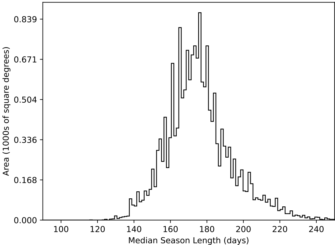
too_100_4v3.4_10yrs WFD all bands: Median Season Length
