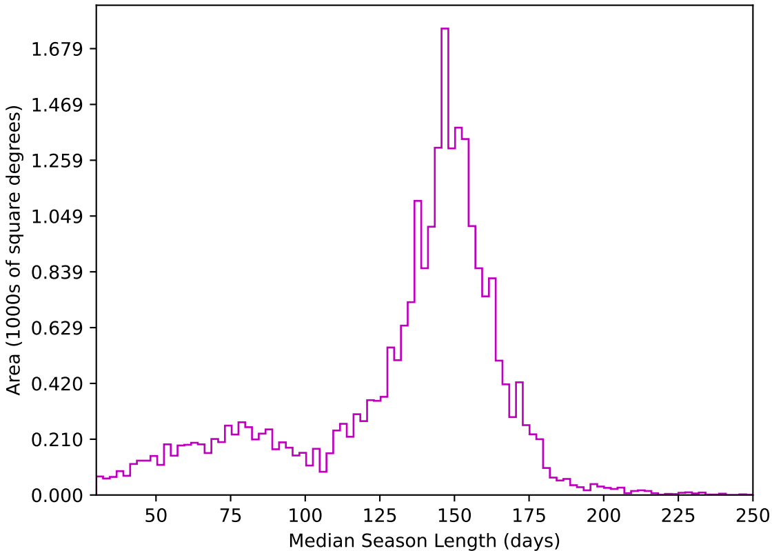
too_100_4v3.4_10yrs All sky z band: Median Season Length
