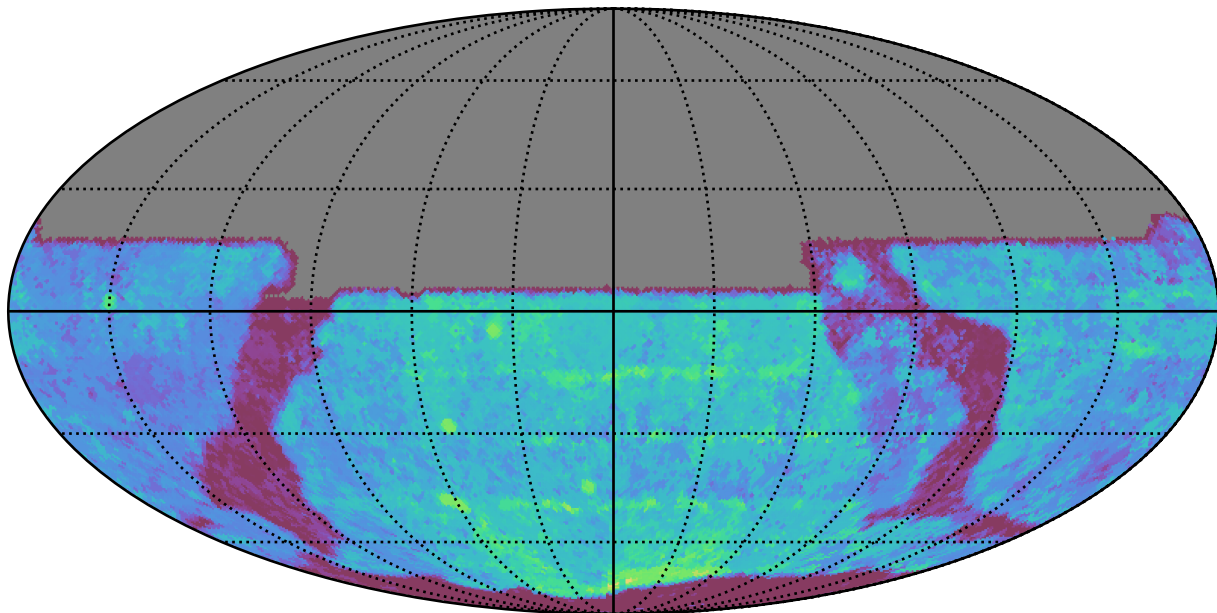
too_100_4v3.4_10yrs All sky y band: Median Season Length
