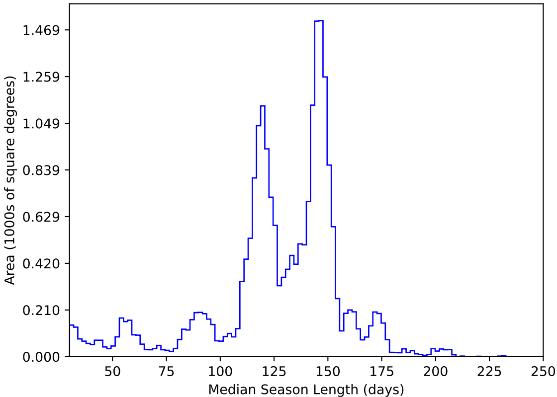
too_100_4v3.4_10yrs All sky y band: Median Season Length
