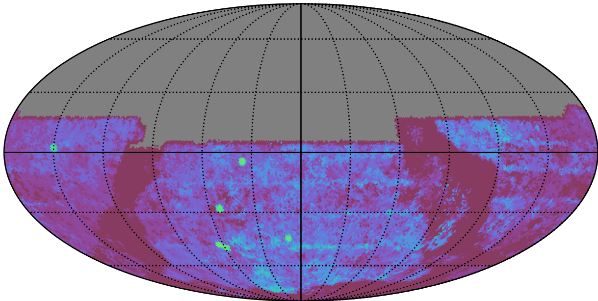
too_100_4v3.4_10yrs All sky u band: Median Season Length
