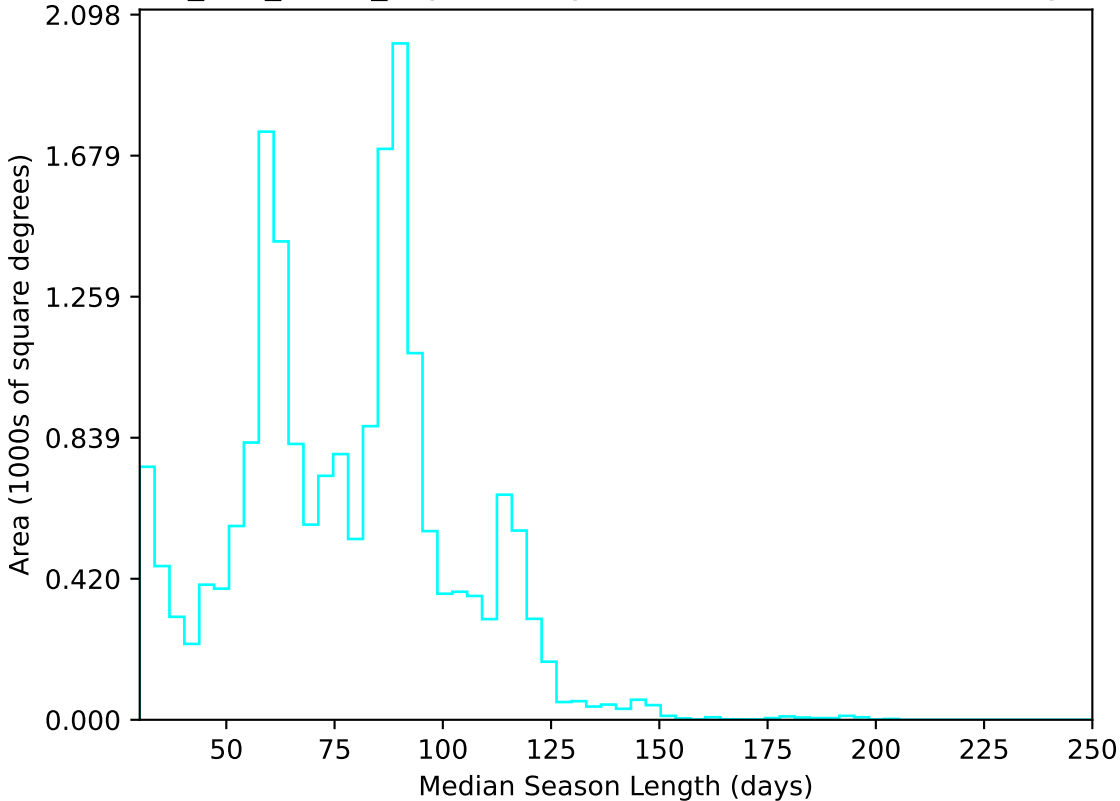
too_100_4v3.4_10yrs All sky u band: Median Season Length
