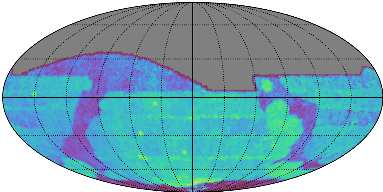
too_100_4v3.4_10yrs All sky i band: Median Season Length
