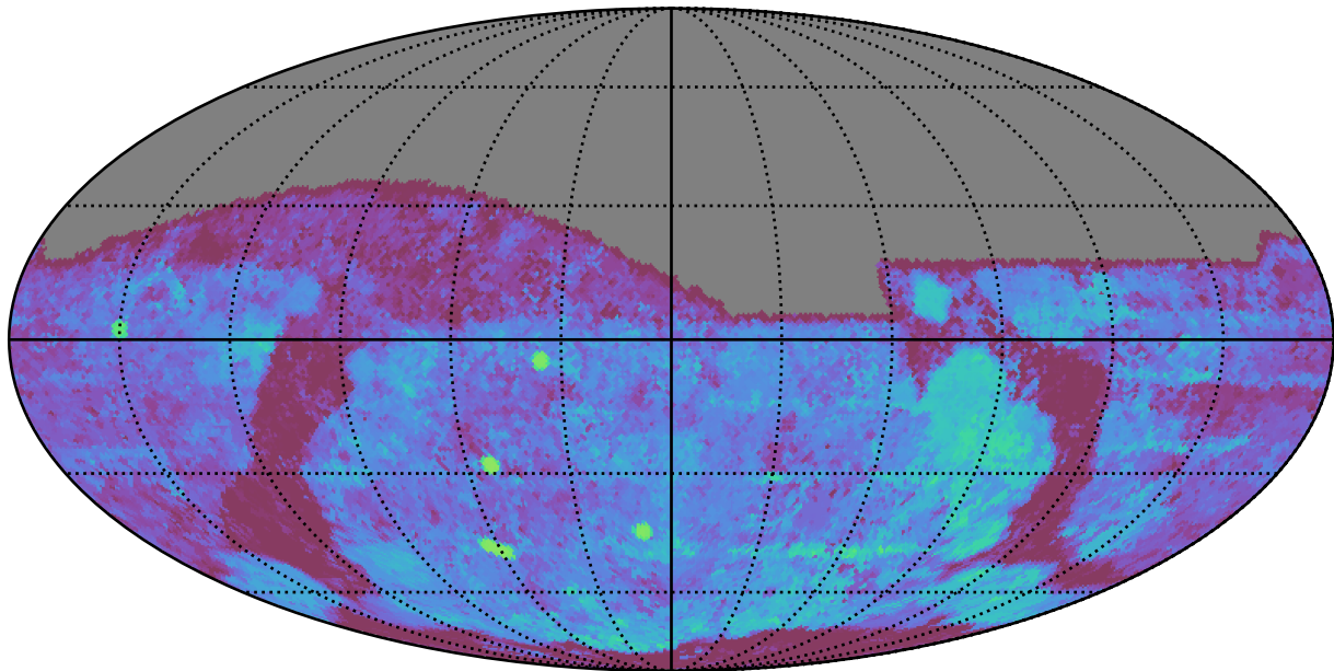
too_100_4v3.4_10yrs All sky g band: Median Season Length
