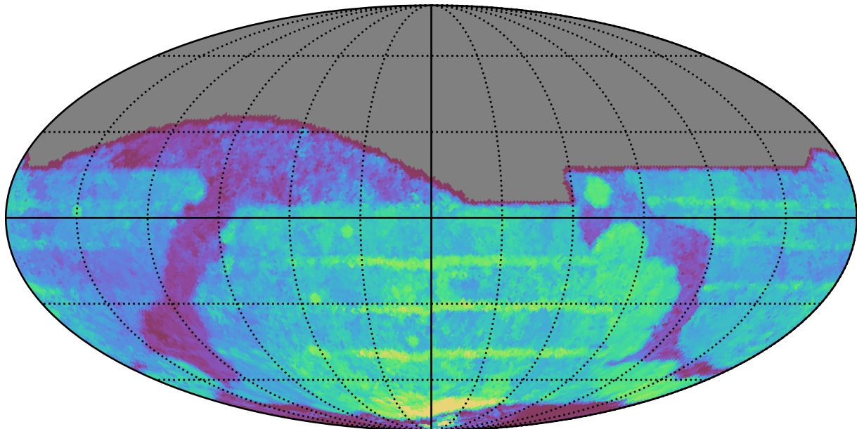
too_100_4v3.4_10yrs All sky all bands: Median Season Length
