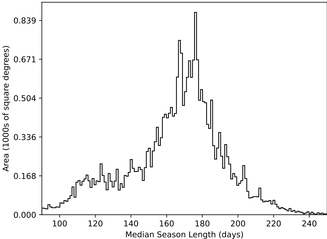
too_100_4v3.4_10yrs All sky all bands: Median Season Length
