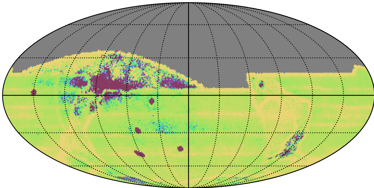
too_100_4v3.4_10yrs All sky: Median Intra-Night Gap
